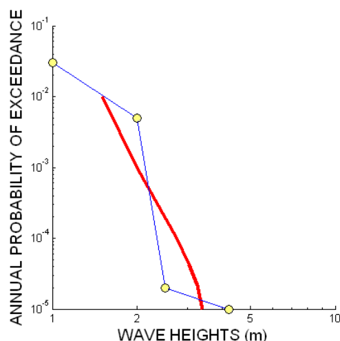
Fig. 1 Tsunami wave height in the reference point versus annual probability of exceedance (1/return period)
